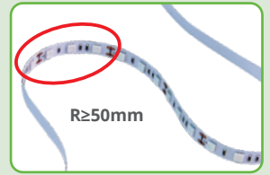
BEND (CORRECT)
